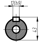
标准轴 Standard output shaft
